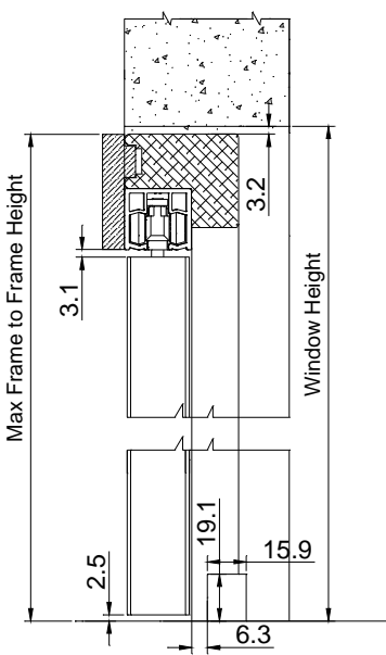
Inside Mount
