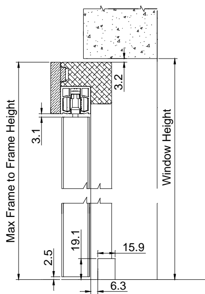
Semi-Inside
