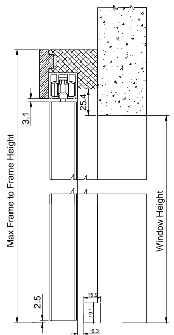
Semi-Inside
