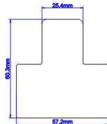
Chamfer T Post 60mm
