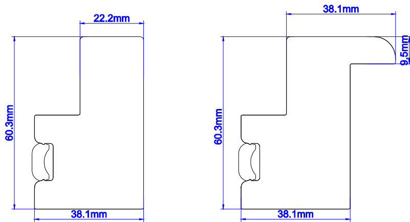
Deep Plain L Frame 60mm Deep Bullnose Z Frame 38mm
